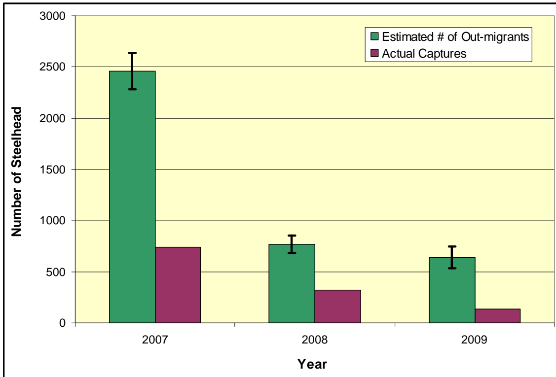
Figure 2. Number of age 1+ steelhead for each trapping year 2007-2009.
