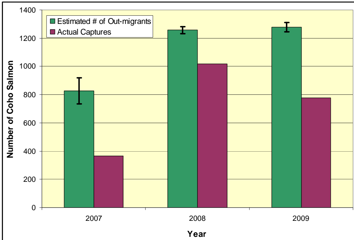
Figure 1. Number of coho salmon smolts for each trapping year 2007-2009.
