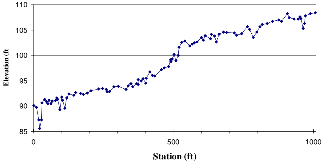
South Fork Cottaneva Creek Long Term Monitoring Longitudinal Profile
