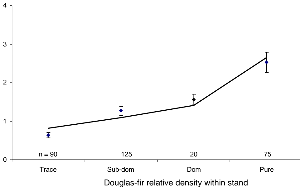
Figure 3. Number of Sonoma tree vole (STV) nests in relation to Douglas-fir relative density within stand. Each point is the mean number of nests across transects, error bars are \pm 1 SEM, n is the number of transects that were surveyed.
