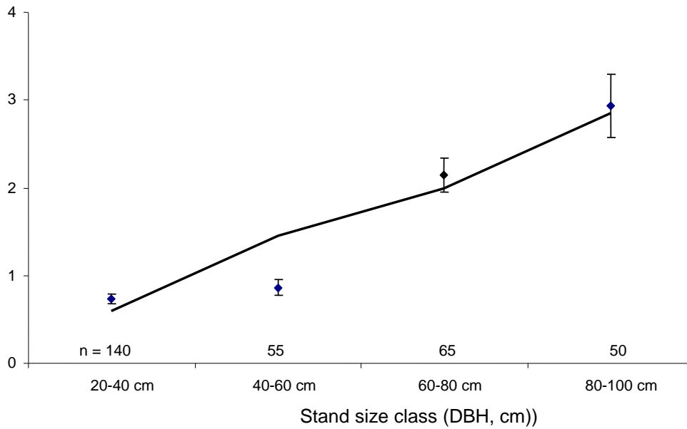
Figure 2. Number of Sonoma tree vole (STV) nests in relation to a stand's tree size class. Each point is the mean number of nests across transects, error bars are \pm 1 SEM, n is the number of transects that were surveyed.
